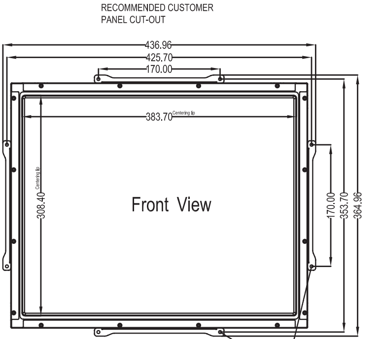
RECOMMENDED CUSTOMER PANEL CUT-OUT
